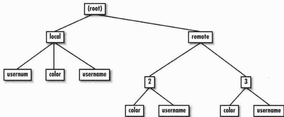
Figure 15-9: Users Environment
