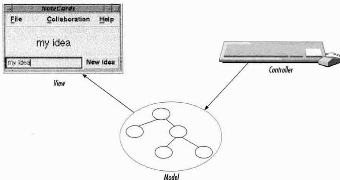
Figure 15-13: Model-View-Controller Paradigm
