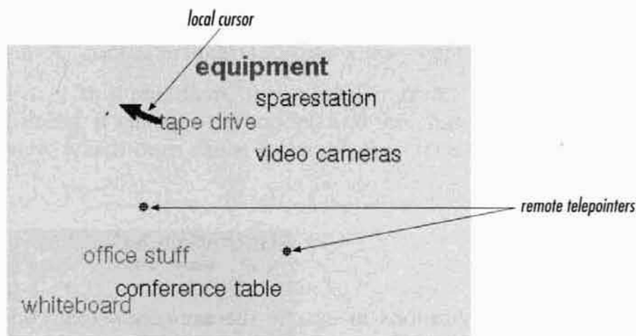
Figure 15-11: GroupKit's Telepointers
