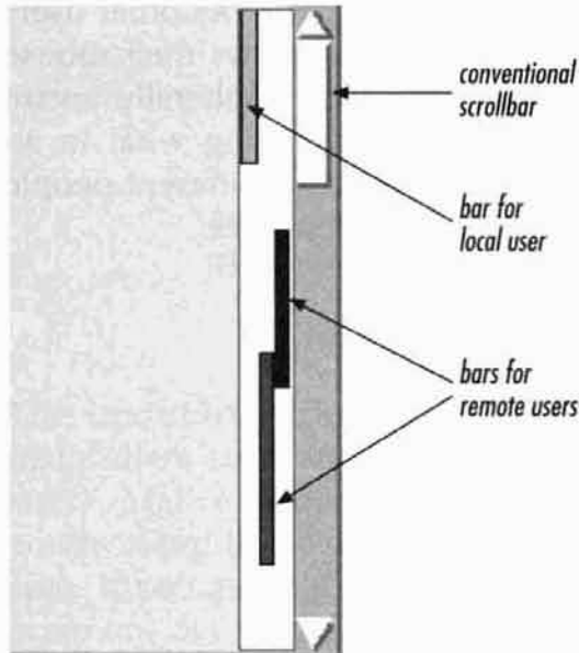
Figure 15-12 Multiuser Scrollbars
